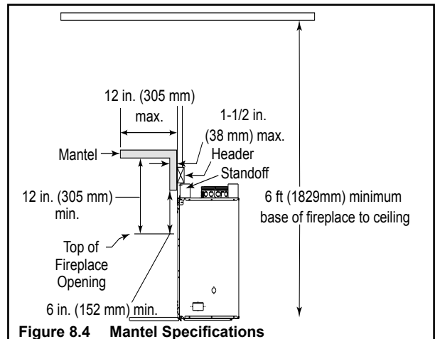
Figure 8.4 Mantel Specifications
