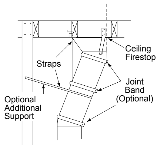
Figure 5.7 Secure the Chimney
