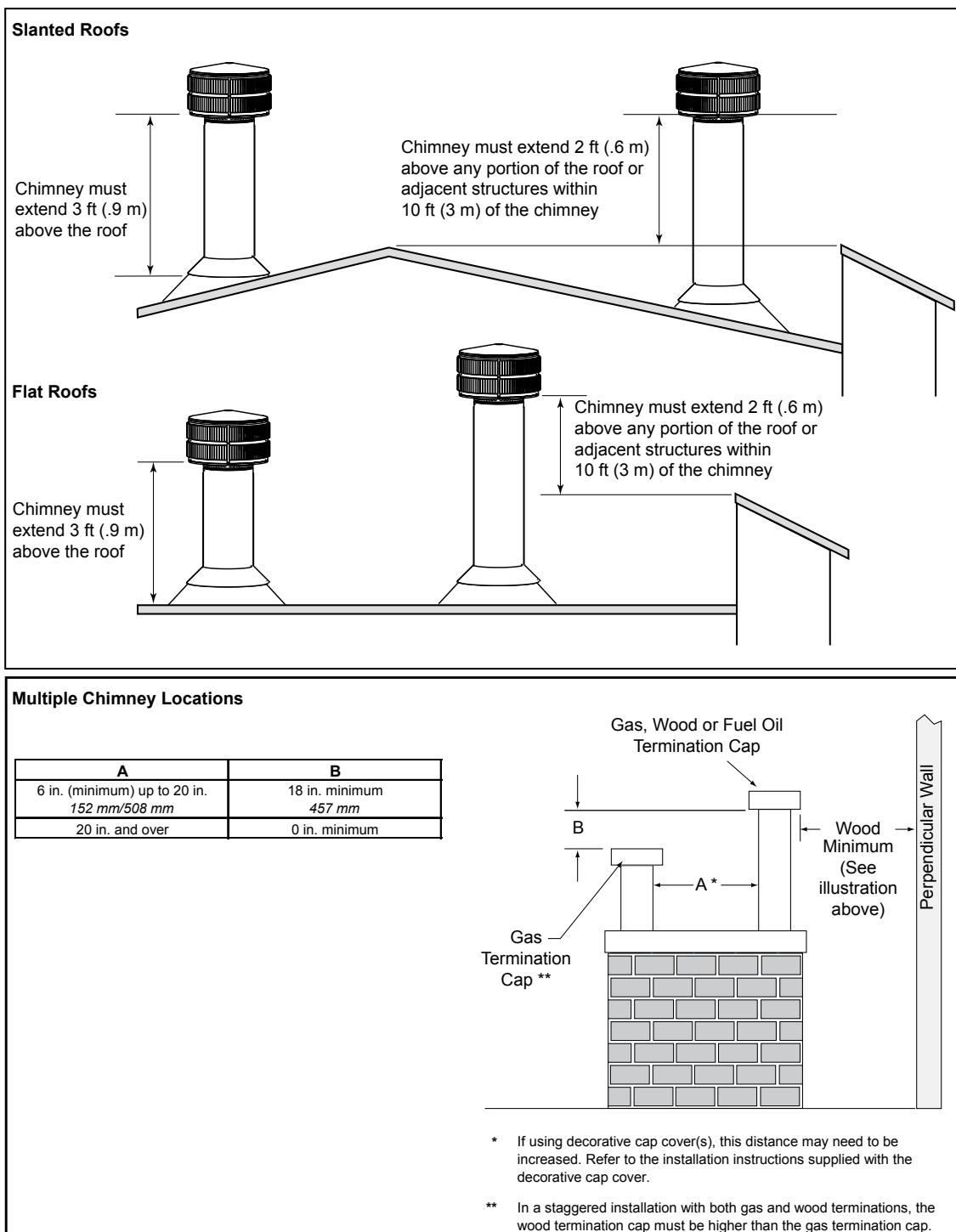
Figure 6.1 Multiple Chimneys
