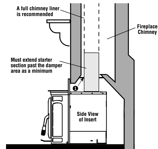
Figure 12 - Positive Flue Connection
