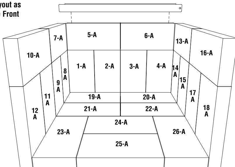
Figure 17 - ML300 Brick Diagram
