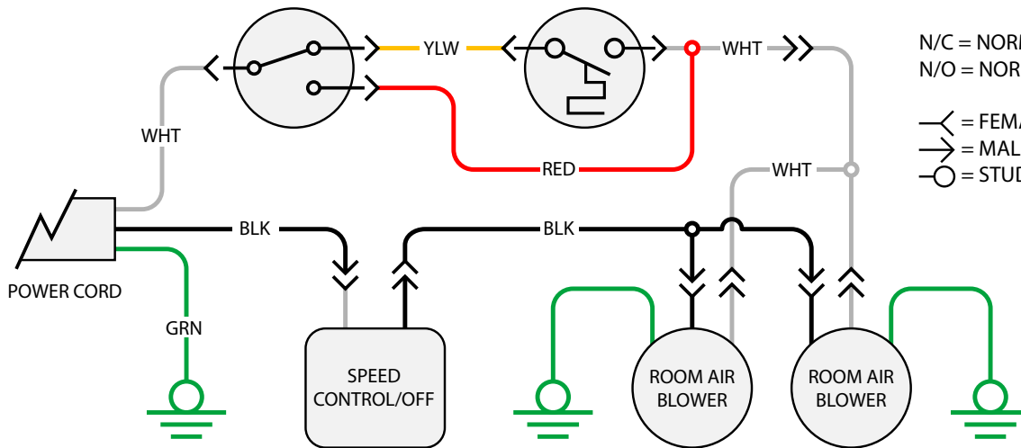
Figure 31B - ML300 Blower Wiring Schematic
