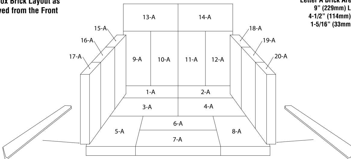
Figure 17 - ML230 Brick
