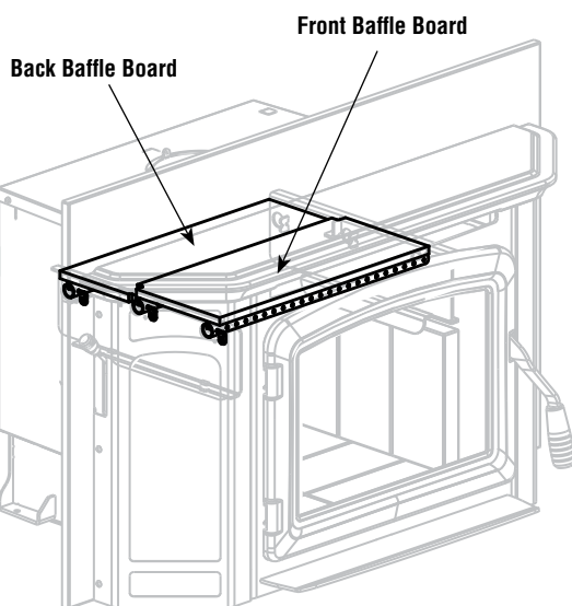
Figure 18 - ML230 Baffle Boards Installed
