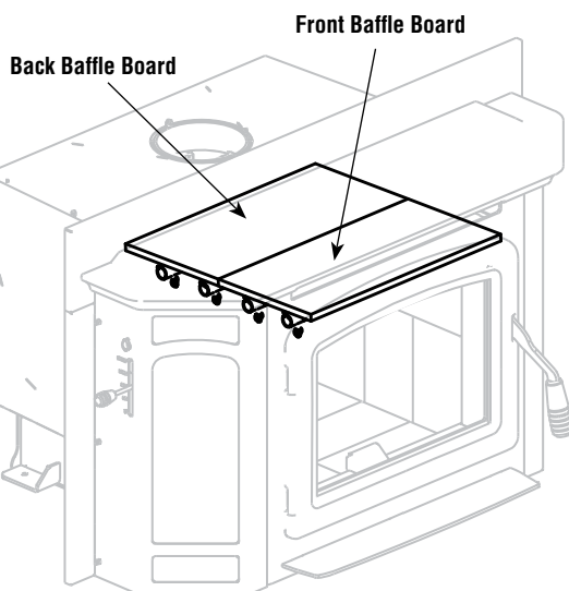
Figure 21 - ML300 Baffle Boards Installed
