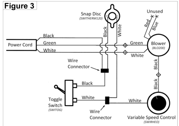
Wiring Diagram
