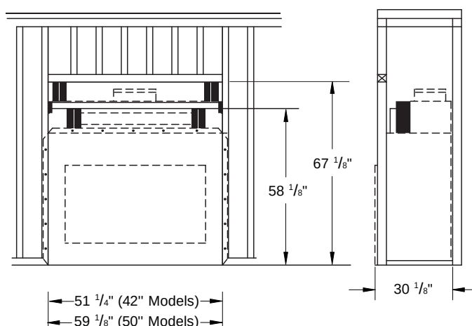
Figure 3 - Framing Dimensions
