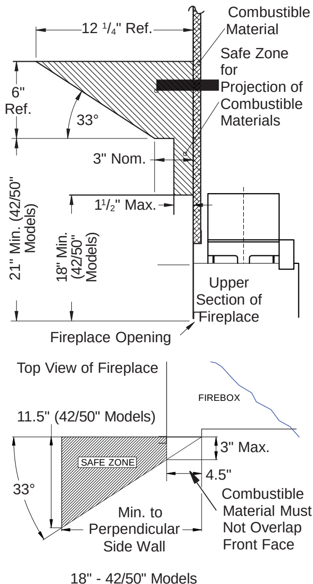
Figure 6 - Mantel Clearances to Combustible Material
