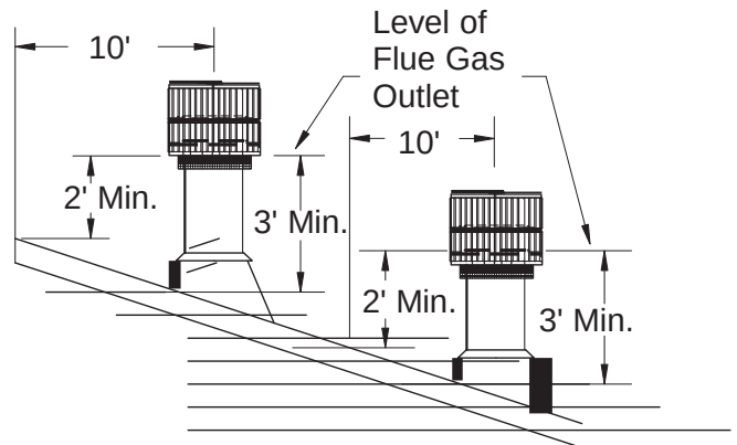
Figure 19 - 10 Foot Rule
