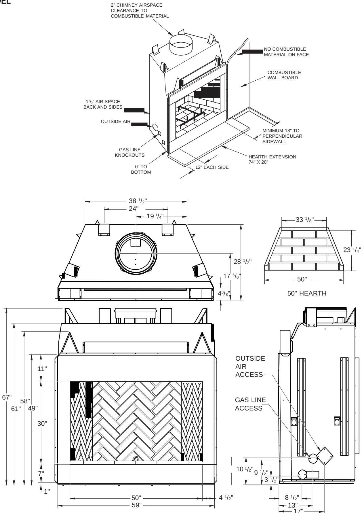
Figure 2 - 50" Models
