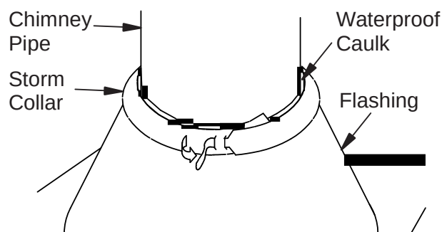
Figure 16 - Storm Collar
