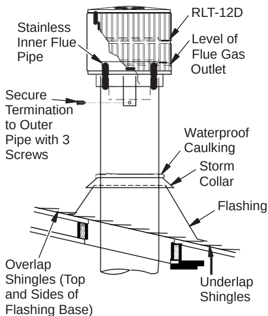
Figure 17 - Termination
