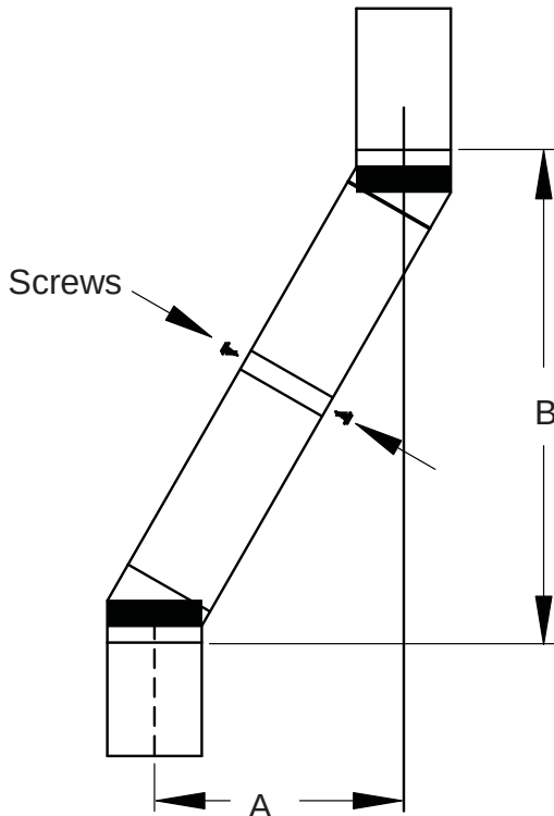
Figure 9 - Elbow Offset
