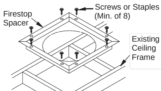
Figure 12 - Firestop Spacer with Living Space Above Ceiling
