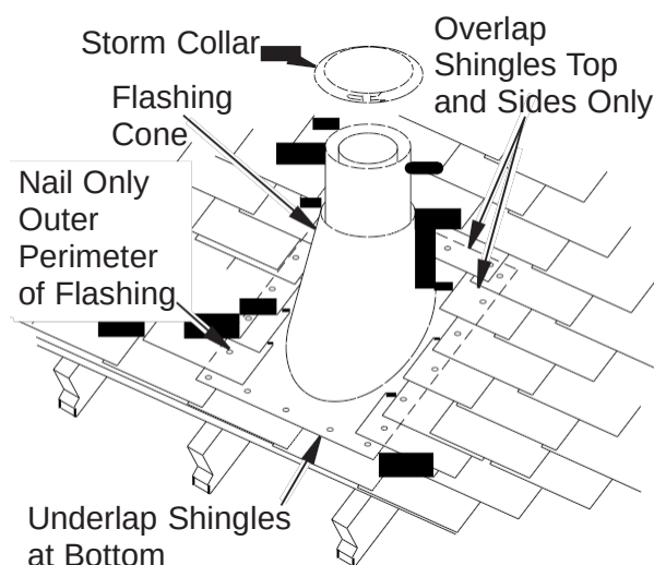
Figure 15 - Flashing Installation
