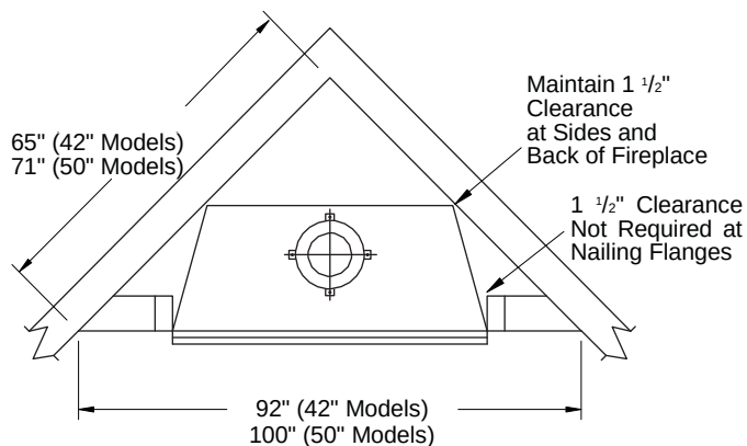
Figure 4 - Corner Installation
