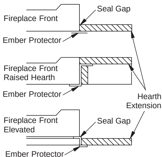
Figure 5 - Hearth Extension
