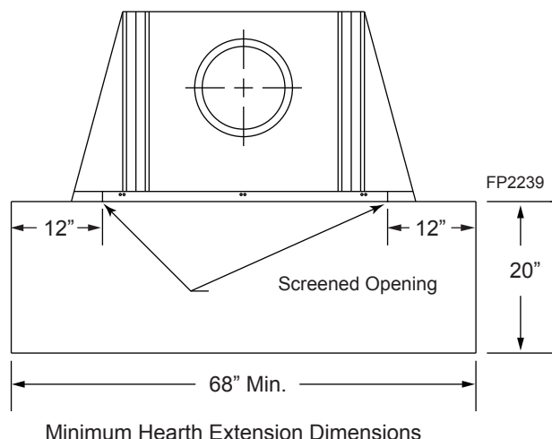
Figure 13 Top View Fireplace and Hearth Extension
