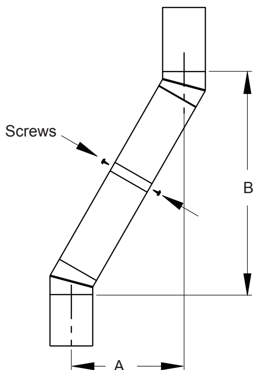
Figure 10 - Elbow Offset
