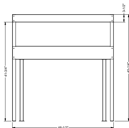
Framing kit dimensions
