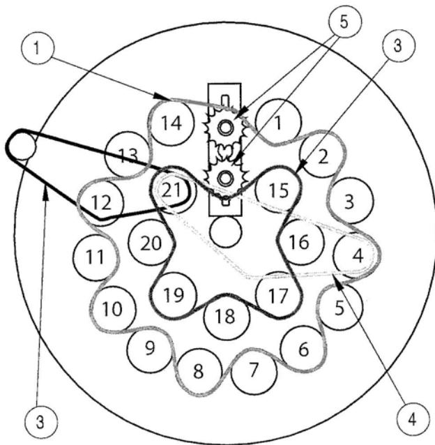
Figure 1 - PC1020 Flue Cleanout Chains
