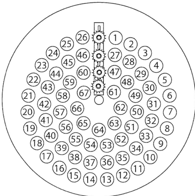
Figure 3 - PC2520 Flue Cleanout Augers
