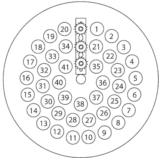
Figure 2 - PC1520 Flue Cleanout Augers
