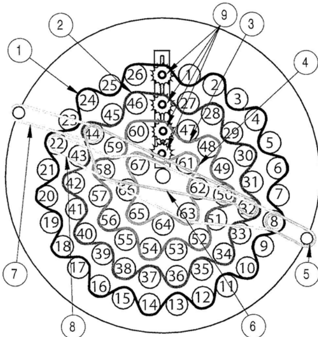
Figure 3 - PC2520 Flue Cleanout Chains
