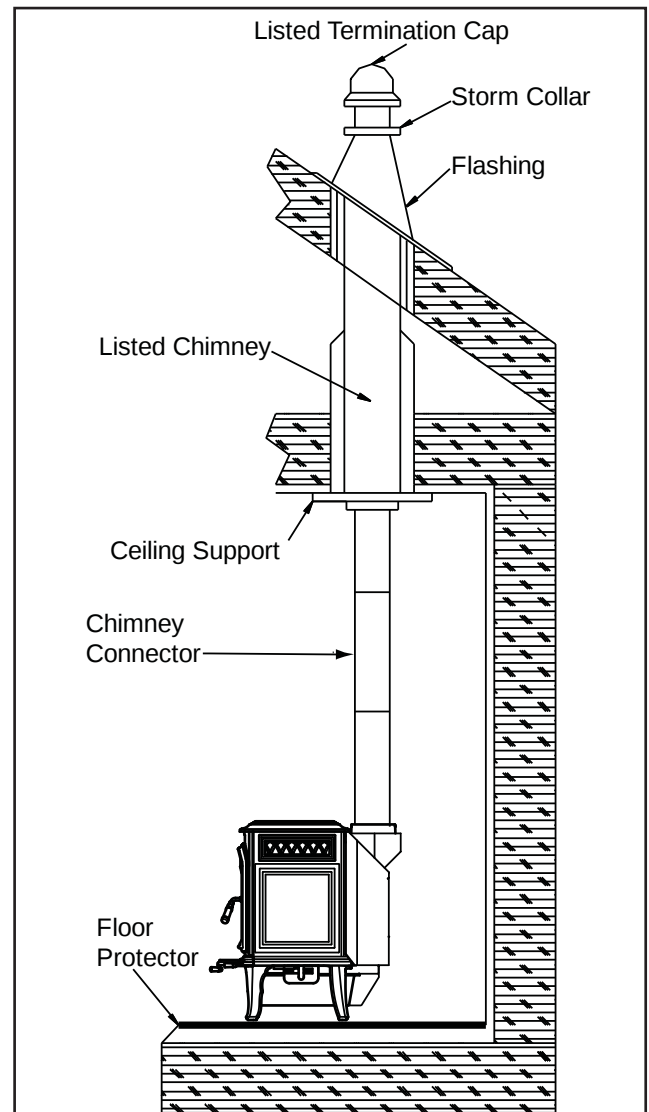
Figure 11.2 - Prefabricated Interior Chimney
