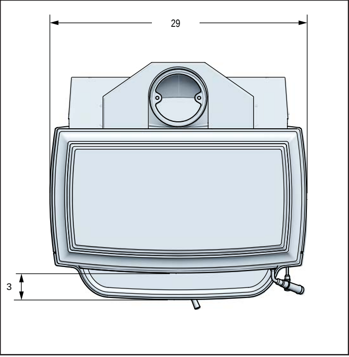
Figure 7.2 Top View
