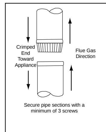
Figure 13.2 Chimney Connector (Stove Pipe)
