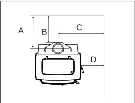
CORNER INSTALLATION
