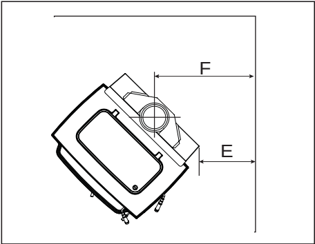
CORNER INSTALLATION
