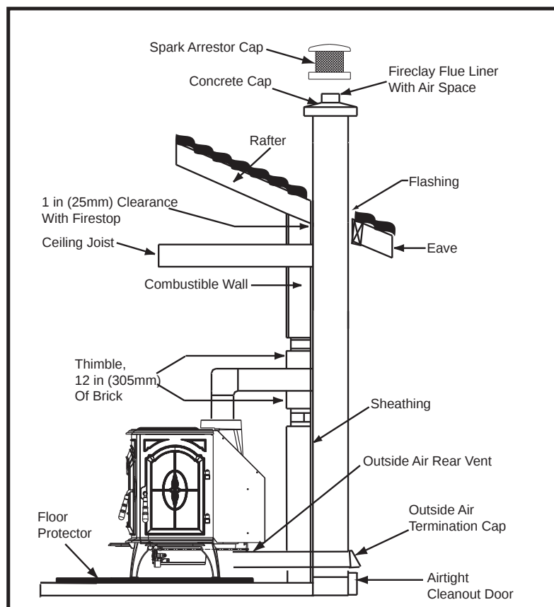
Figure 8.1 Masonry Chimney
