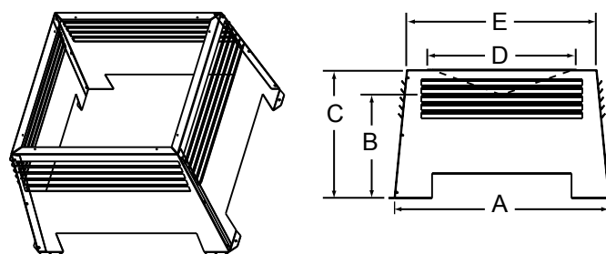
LDS-BV Decorative Shroud
