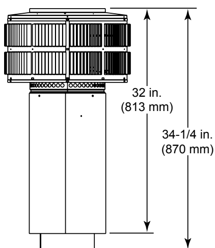
TV342 Top Vent Round Termination Cap
