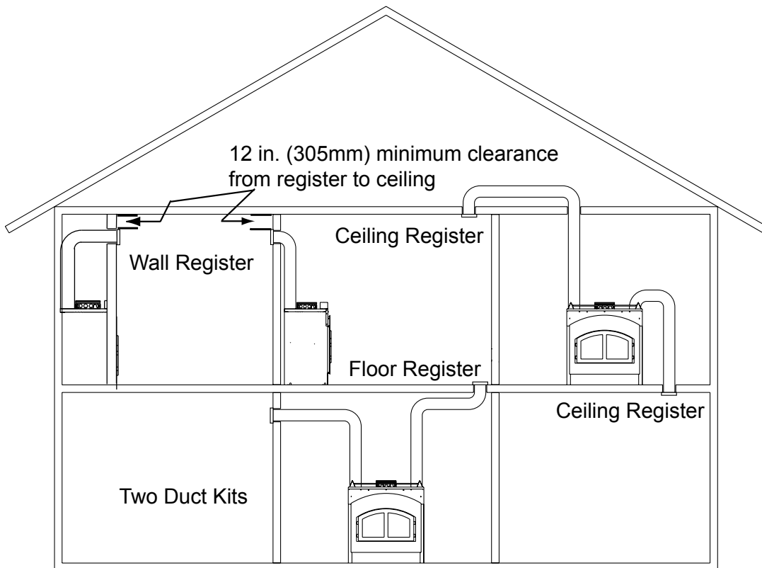
Figure 3.15 Minimum Clearances to Combustibles
