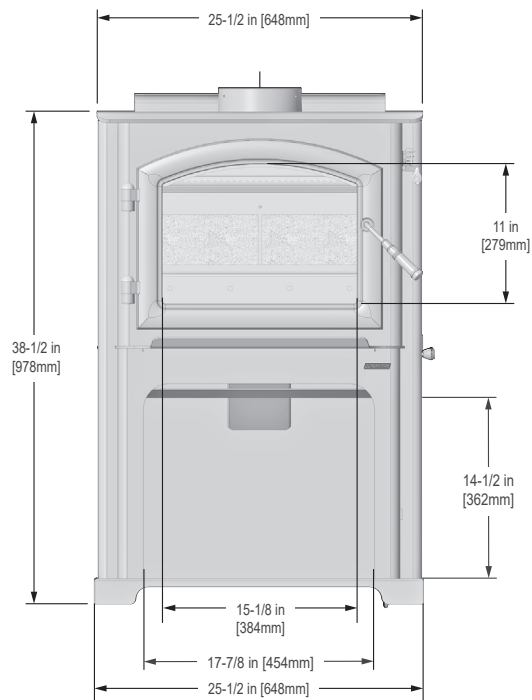
Figure 8.1 - Front View
