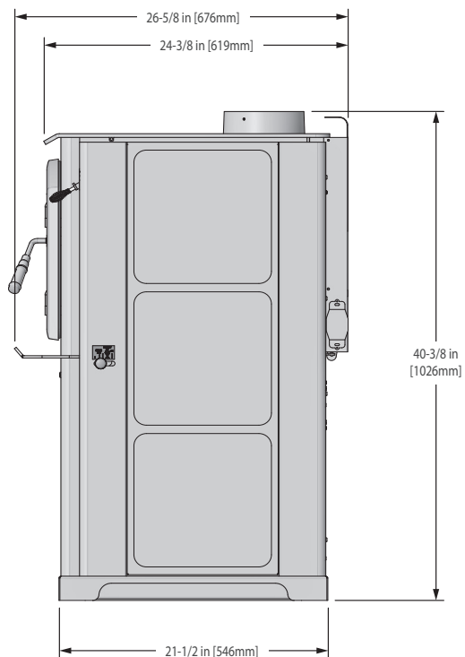
Figure 8.3 - Side View
