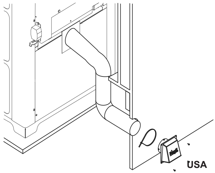
Figure 16.2 - Floor Installation
