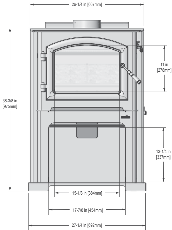
Figure 8.1 - Front View
