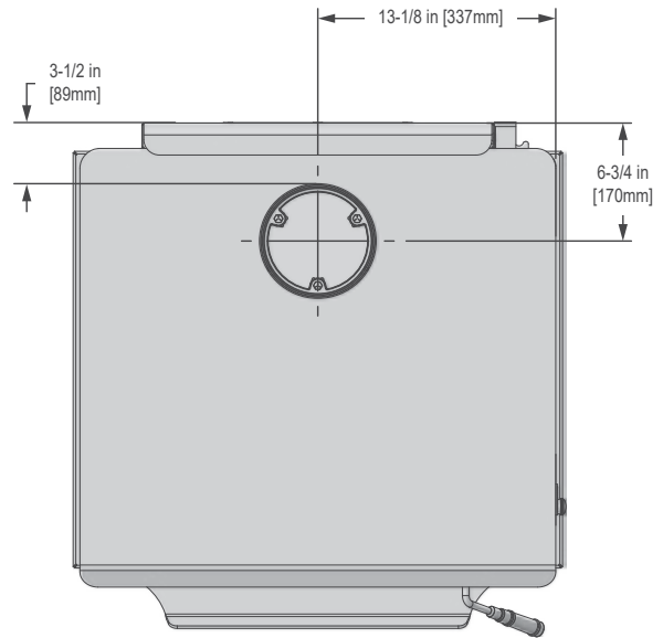
Figure 8.2 - Top View
