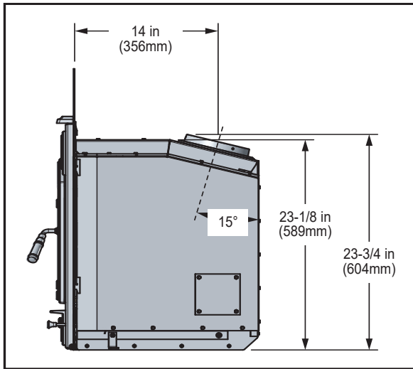
Figure 9.1 - Side View with Flat Surround
