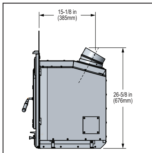
Figure 9.3 - Side View with Flat Surround and Optional 15 Degree Adapter (DV-6DLR-E15ADSS)
