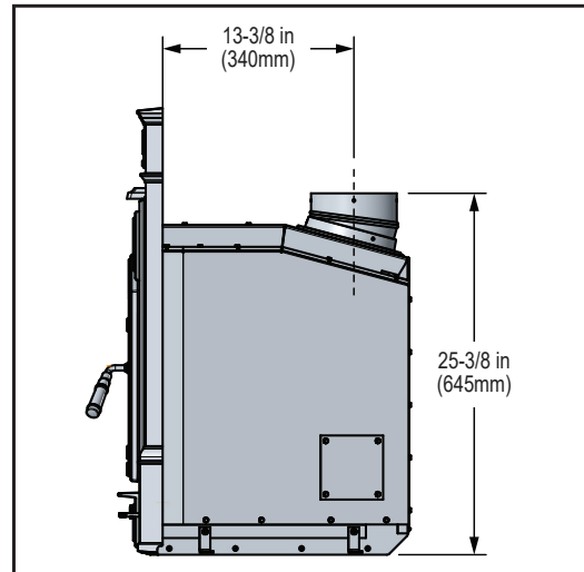
Figure 9.5 - Side View with Cast Surround and Optional 15 Degree Adapter (DV-6DLR-E15ADSS)
