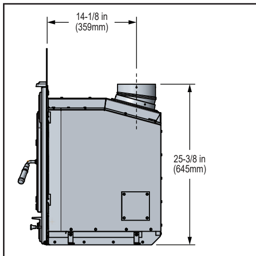
Figure 9.2 - Side View with Flat Surround and Optional 15 Degree Adapter (DV-6DLR-E15ADSS)
