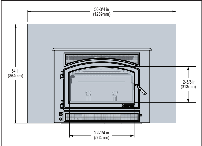
Figure 8.3 - Front View with Large Flat Surround (SP2-5134)
