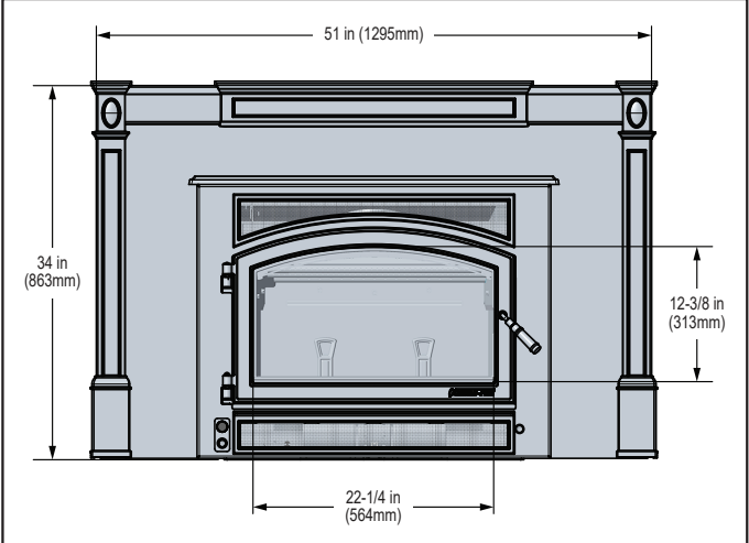
Figure 8.6 - Front View with Large Flat Surround (CT2-5134) with Cast Trim (811-0930)
