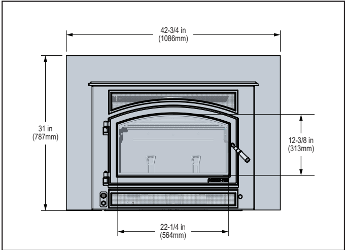
Figure 8.2 - Front View with Small Flat Surround (SP2-4331)
