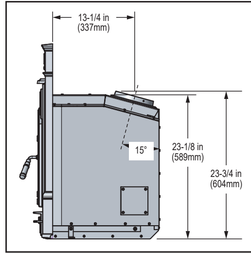
Figure 9.4 - Side View with Cast Surround
