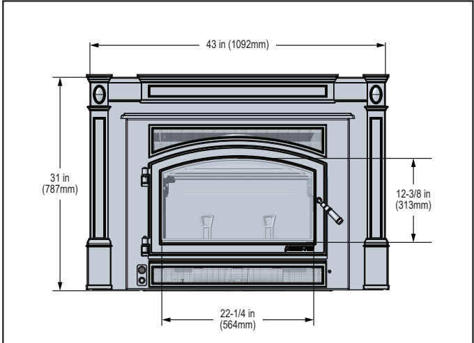
Figure 8.5 - Front View with Small Flat Surround (CT2-4331) with Cast Trim (811-0930)
