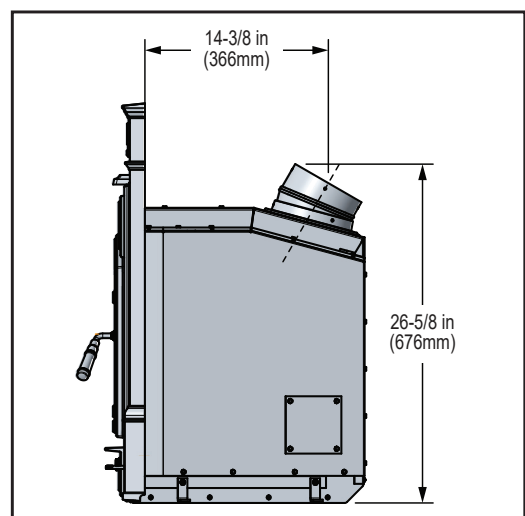
Figure 9.6 - Side View with Cast Surround and Optional 15 Degree Adapter (DV-6DLR-E15ADSS)
