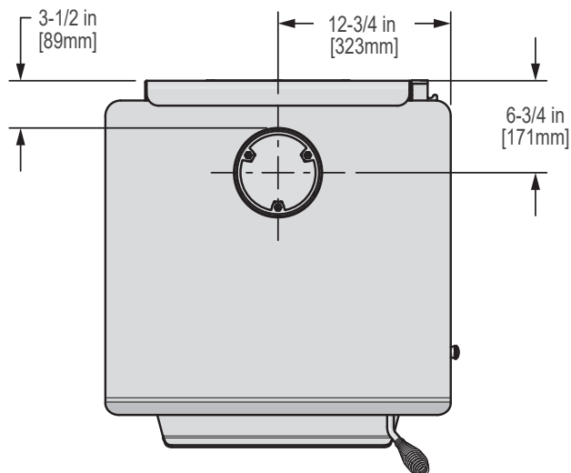
Figure 8.2 - Top View
