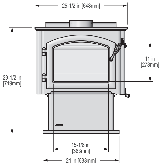
Figure 8.1 - Front View
