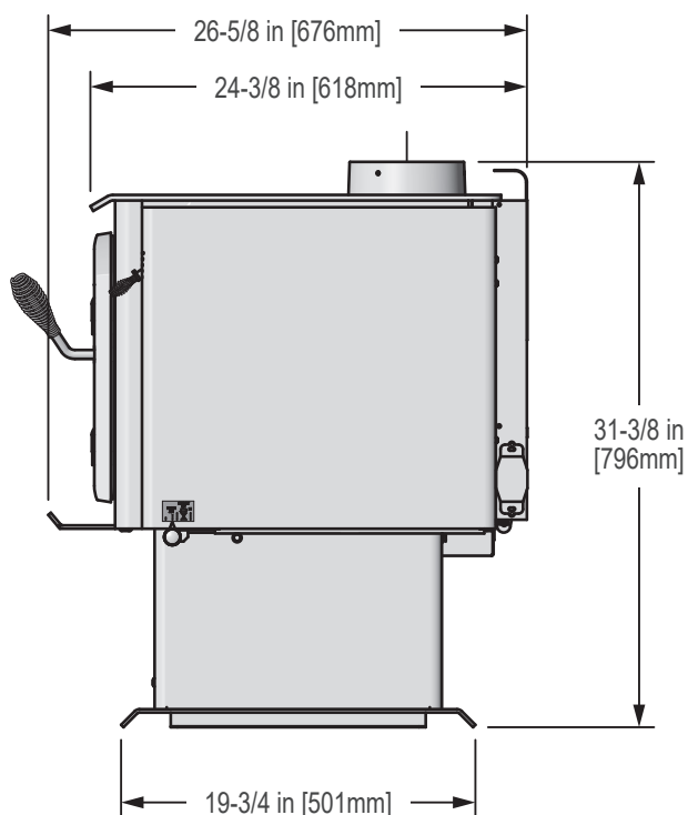
Figure 8.3 - Side View
