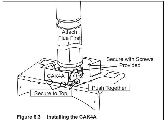
Figure 6.3 Installing the CAK4A
