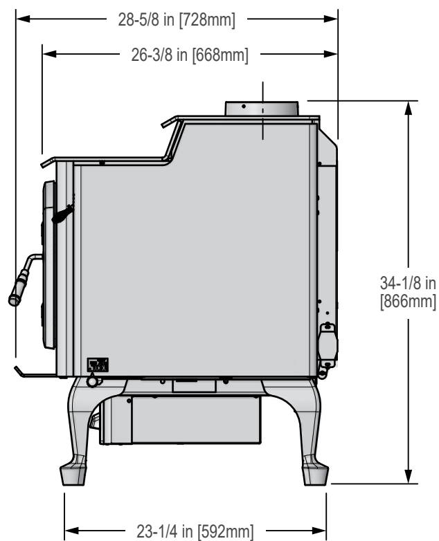
Figure 11.2 - Side View
