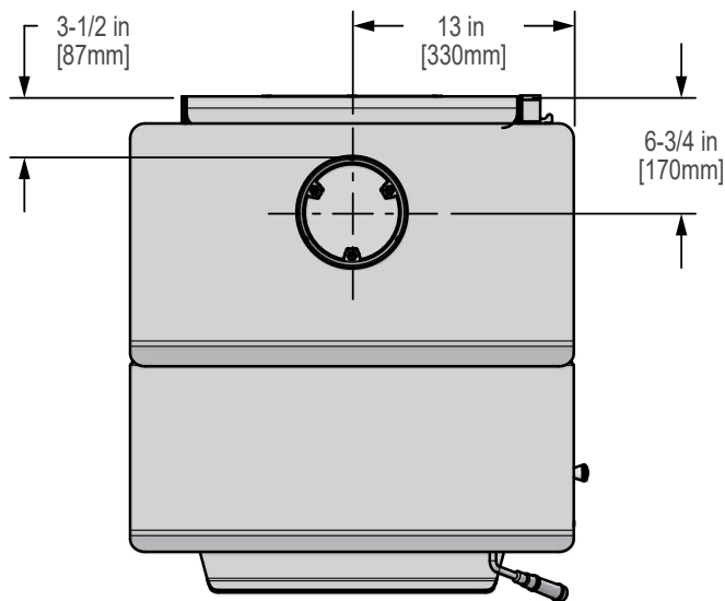
Figure 10.3 - Top View
