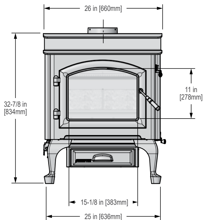
Figure 11.1 - Front View
