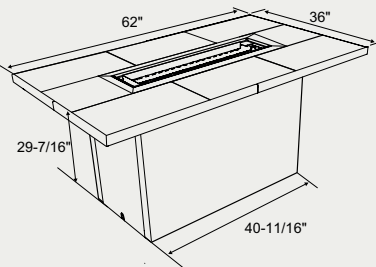
PTO30IST Island Firetable
