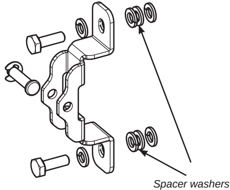
Spacer washers
