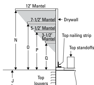
MANTEL CLEARANCES - SIDE VIEW
