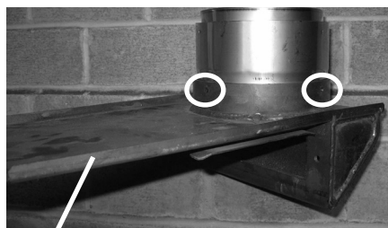
Flue Adaptor
