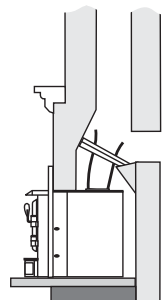
1) Positive Flue Connection with Cleanout
