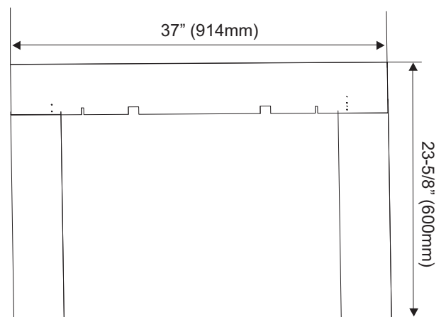
CI1200 Custom - Minimum Dimensions
