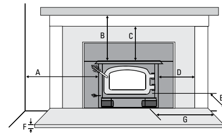
Hearth Heater Minimum Fireplace Openings
