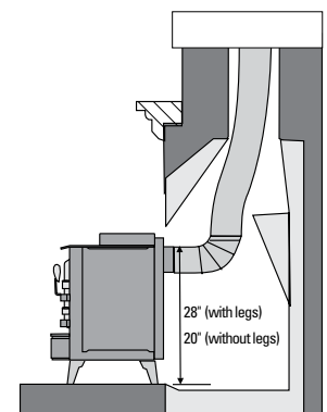
Hearth Heater Minimum Fireplace Openings
