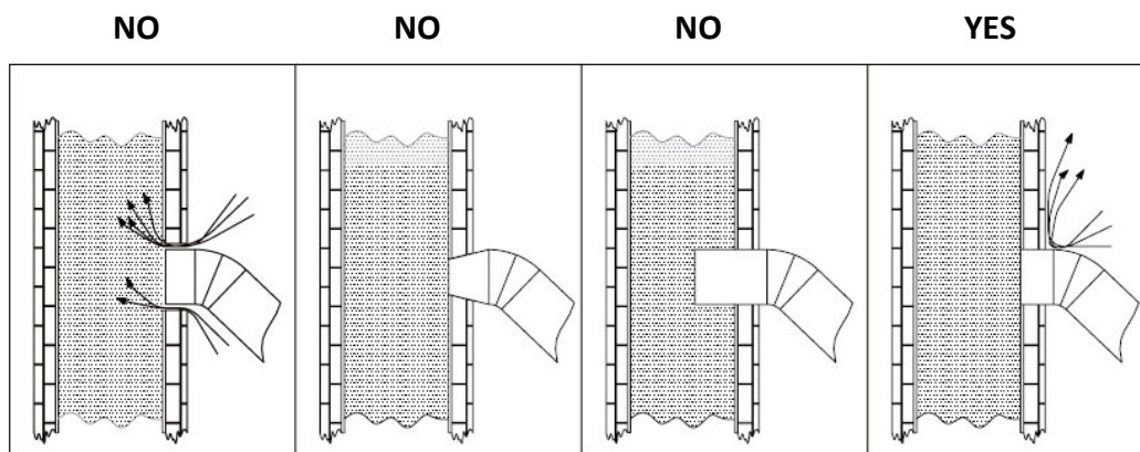
Picture 7 - Examples of correct and incorrect connection of the chimney.
