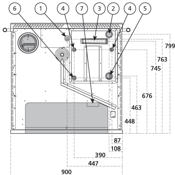
Picture 15 1 Connection thermostat detector Ø 1/2" female 5 Return connection Ø 1 1/4 female 2 Going connection Ø 1 1/4 female 6 Connection discharge Ø 1/2" female 3 Connection for thermal discharge detector Ø 1/2" female 7 External air intake (optional) 4 Connections for thermal discharge circuit Ø 1/2" male
