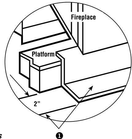
Figure 14 - Hearth Extension Requirements
