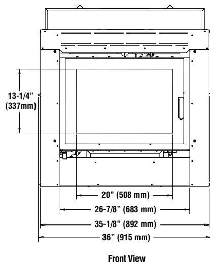
Figure 16 - Framing Dimensions
