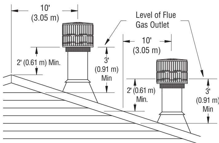
Figure 22 - 10 Foot Rule
