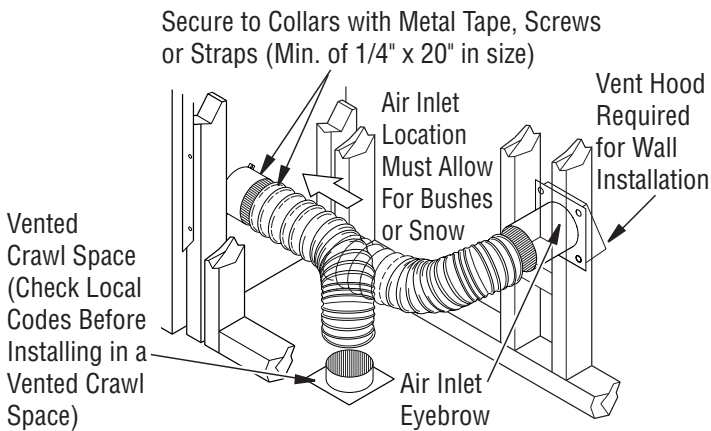
Figure 10 - Outside Air Kit
