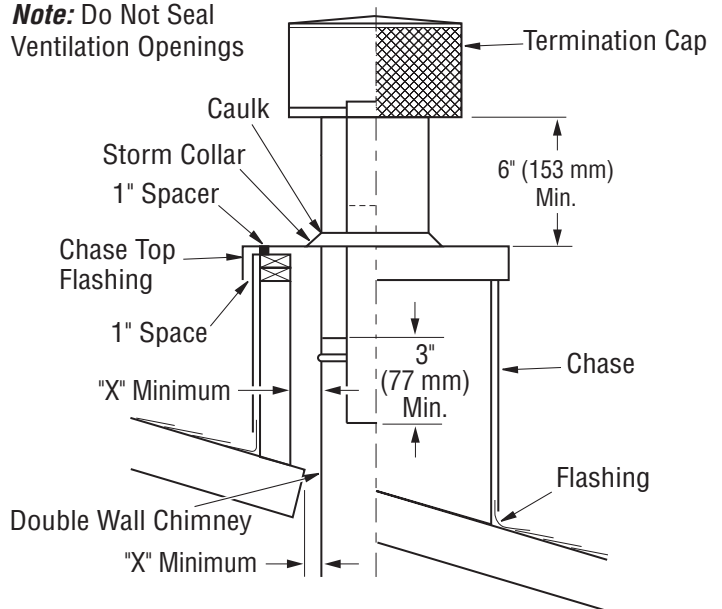
Figure 31 - Chase Installation
