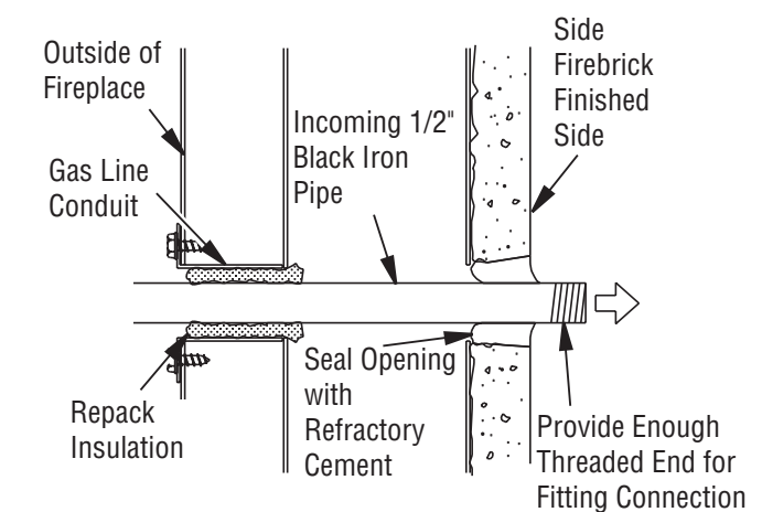
Figure 39 - Gas Line Installation
