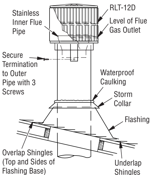
Figure 20 - Termination
