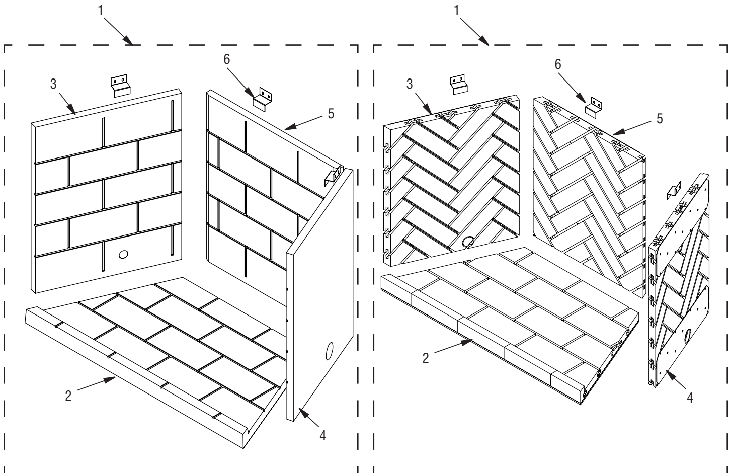
Stacked Refractory
