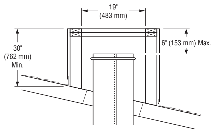
Figure 23 - Constructing Chase
