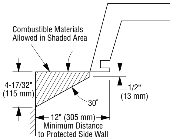
Figure 9 - Mantel Clearances to Combustible Materials
