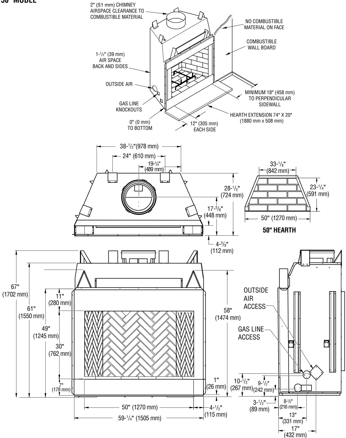
Figure 3 - 50" Models
