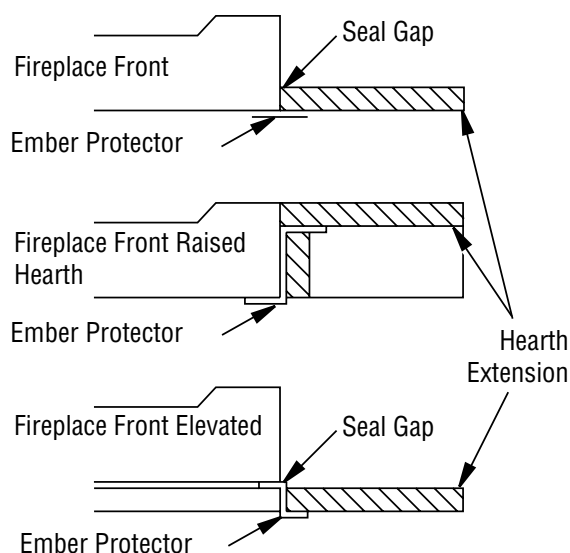
Figure 6 - Hearth Extension
