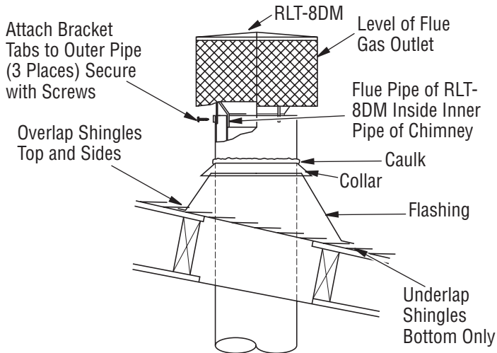
Figure 18 - Termination
