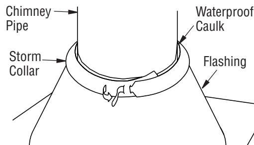
Figure 17 - Storm Collar
