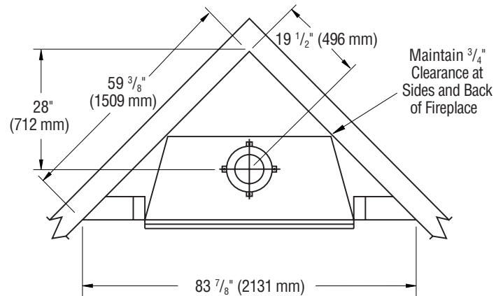
Figure 2 - Corner Installation
