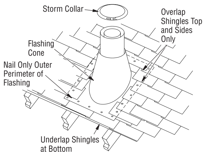
Figure 16 - Flashing Installation
