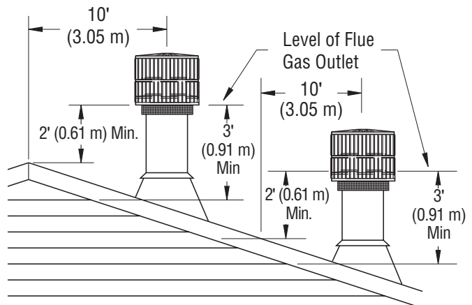
Figure 20 - 10 Foot Rule
