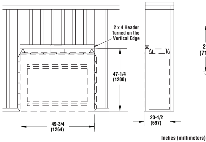
Parallel Framing Dimensions
