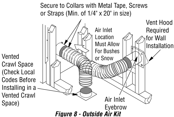
Figure 8 - Outside Air Kit
