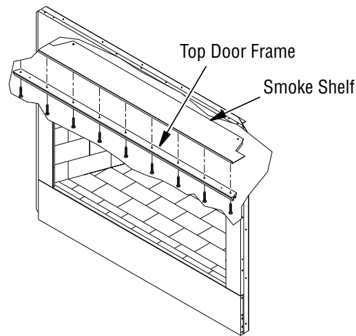
Figure 39 - Installing Top Door Frame
