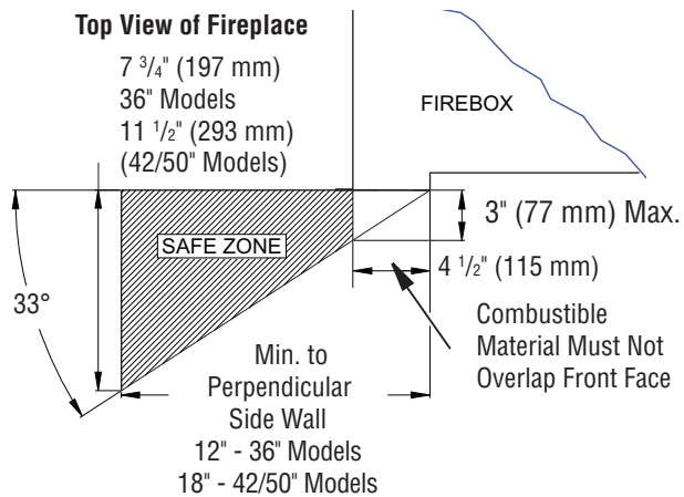
Figure 7 - Mantel Clearances to Combustible Material
