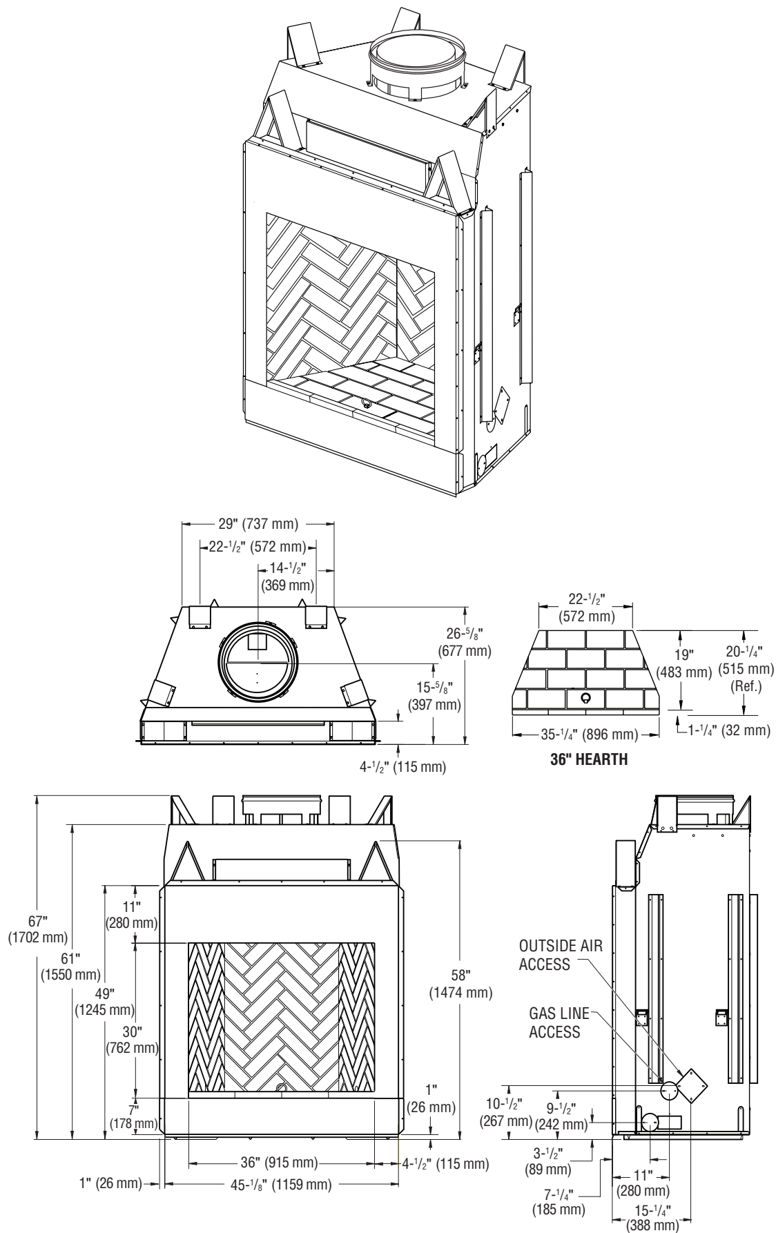
Figure 1 - 36" WRT6036RS, WRT6036IS, WRT6036RH and WRT6036IH
