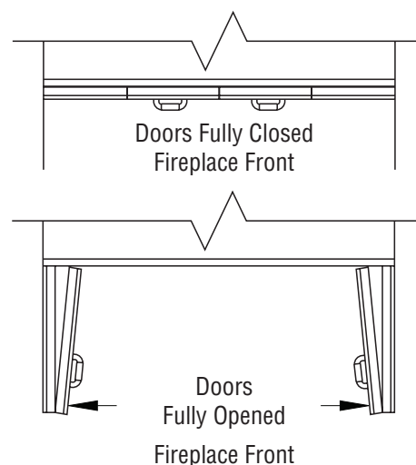
Figure 43 - Bi-Fold Glass Doors
