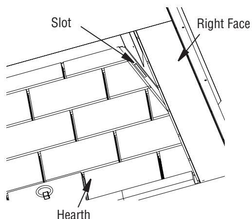
Figure 32 - Slots for Firebrick Walls
