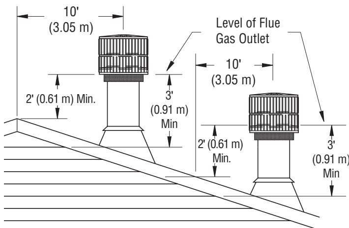
Figure 20 - 10 Foot Rule
