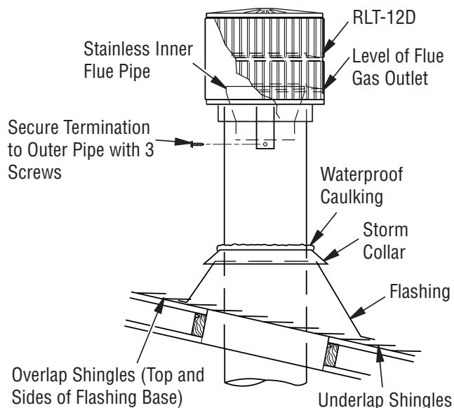
Figure 18 - Termination
