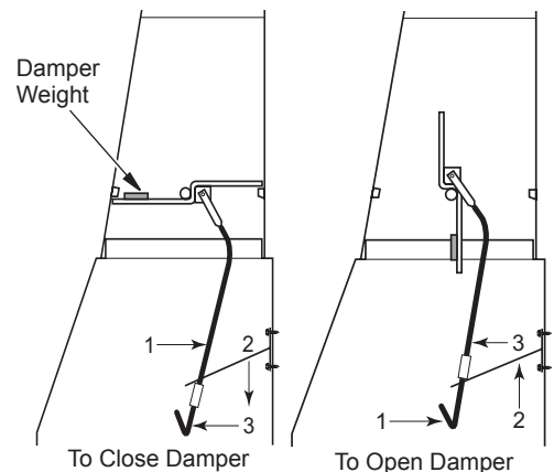
Figure 25 - Damper Rod
