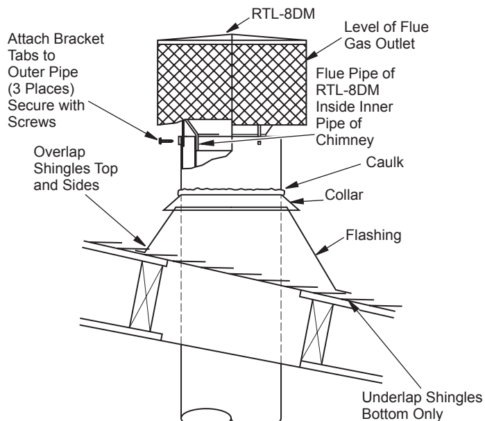
Figure 17 - Termination
