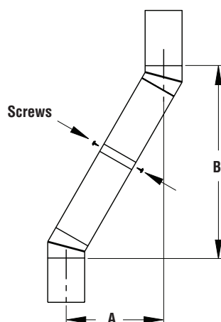
Figure 14 - Elbow Offset
