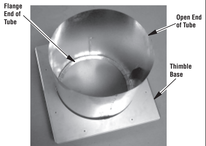
Figure 13 - Attaching Adjustable Thimble
