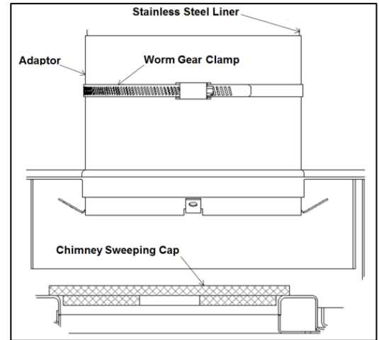
Figure 17: Liner Adaptor Installation
