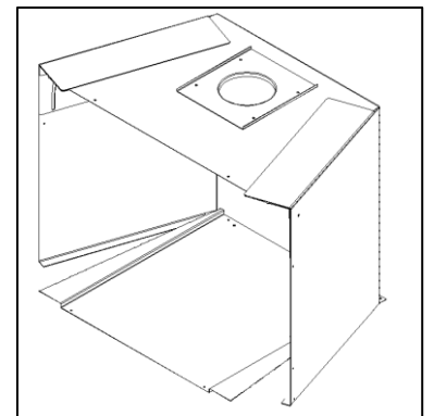
Figure 16: Circulating Chamber Assembly
