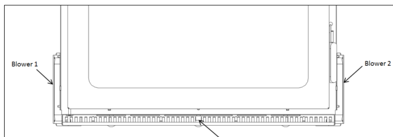
Figure 21: Location of Electric Wiring
