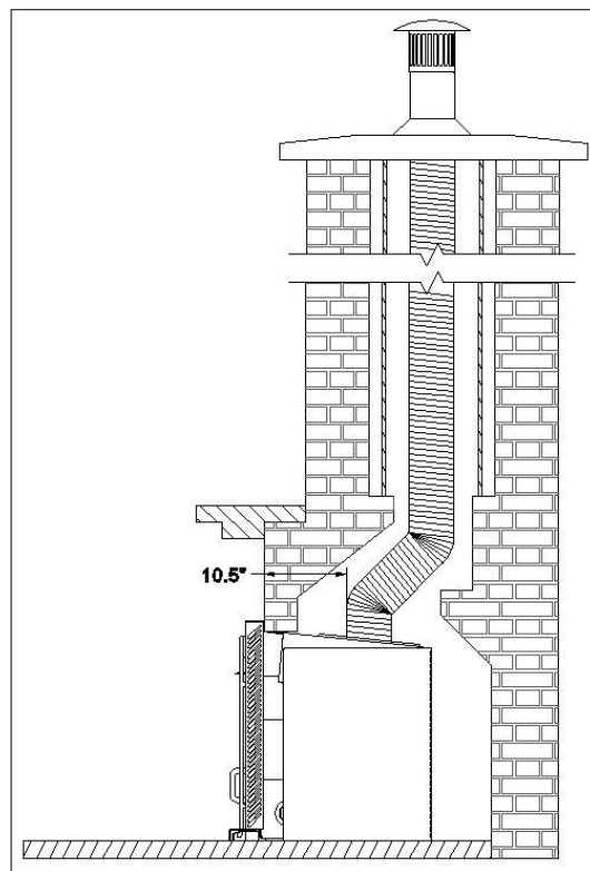
Figure 20: Fusion Installation
