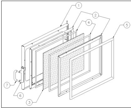
Figure 26: Exploded View of Door Assembly
