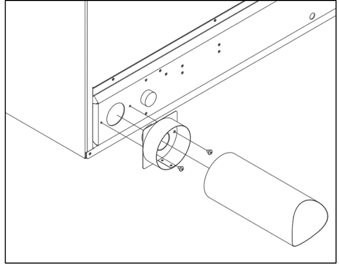
Figure 4-1: Novo Fresh Air Connection
