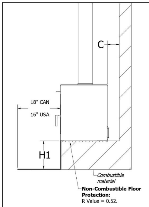
Figure 3-8: Novo Installation at H1
