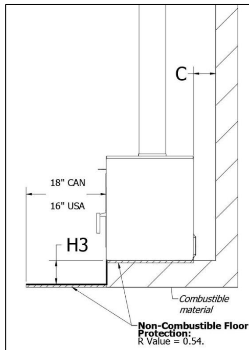
Figure 3-7: Novo Installation at H3
