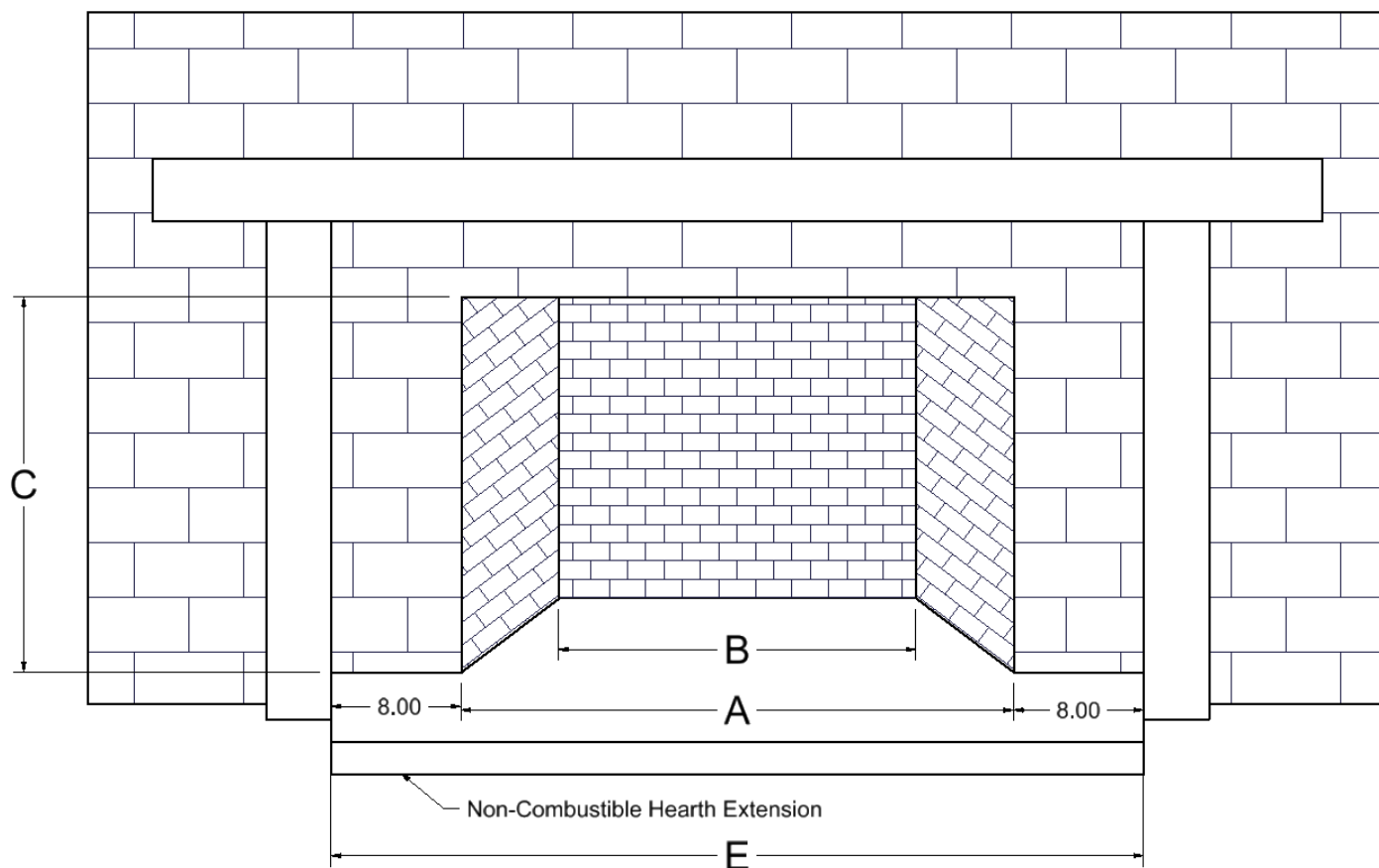
Figure 3-1: Minimum Opening Dimensions – Front View
