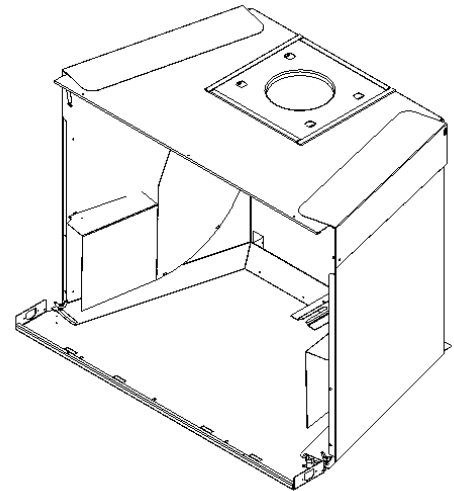
Figure 2-9: Circulating Chamber
