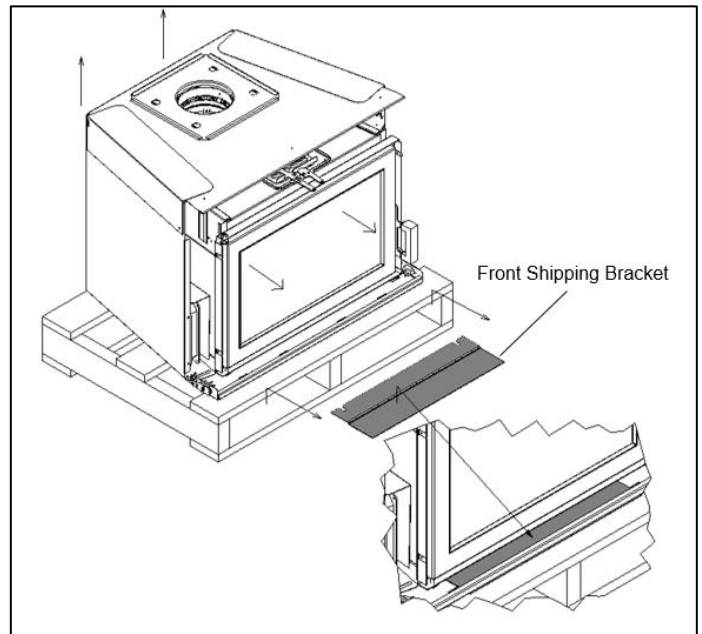
Figure 3-4: FUSION Front Shipping Bracket
