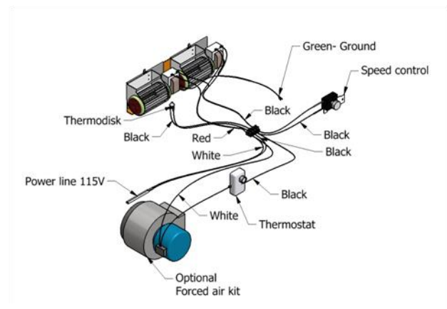
Figure 23 – Fan Wiring for Optional Forced Air Kit
