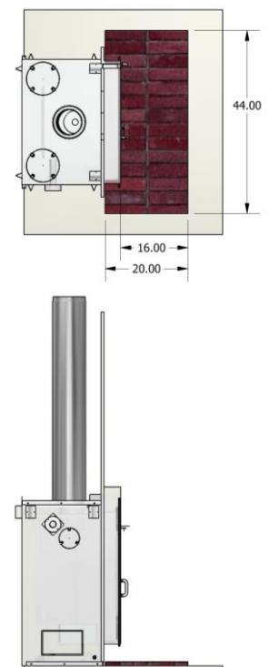
Figure 17 – Hearth Extension
