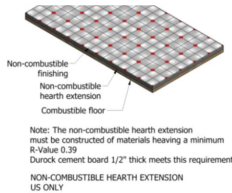
Figure 18 – Non-Combustible Hearth Extension. U.S. Installations Only
