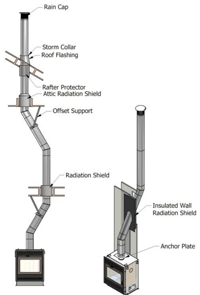
Figure 23 – Chimney Installation
