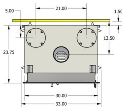
Figure 10 – Parallel Installation
