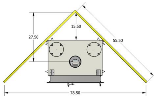
Figure 11 – Corner Installation
