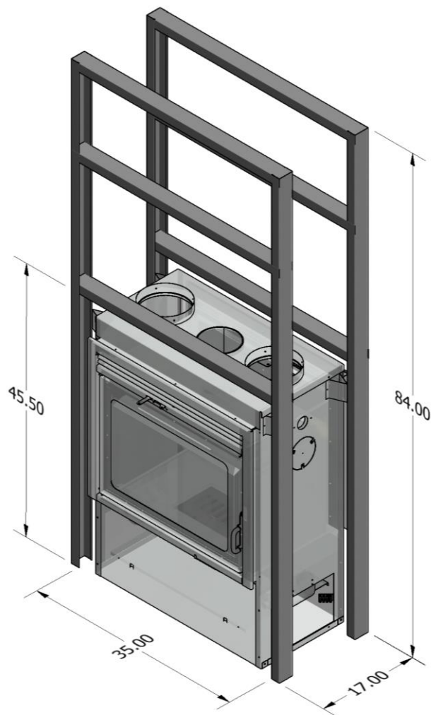
Figure 12 – Framing dimensions
