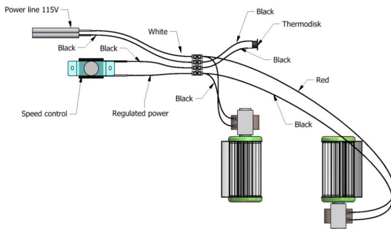
Figure 17 – Blower Kit Wiring
