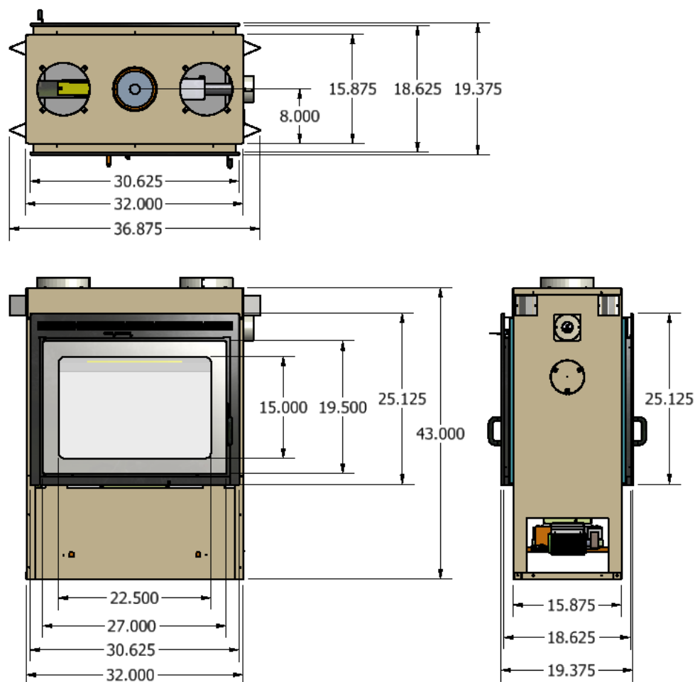
Figure 9 – Dimensions of the Duet
