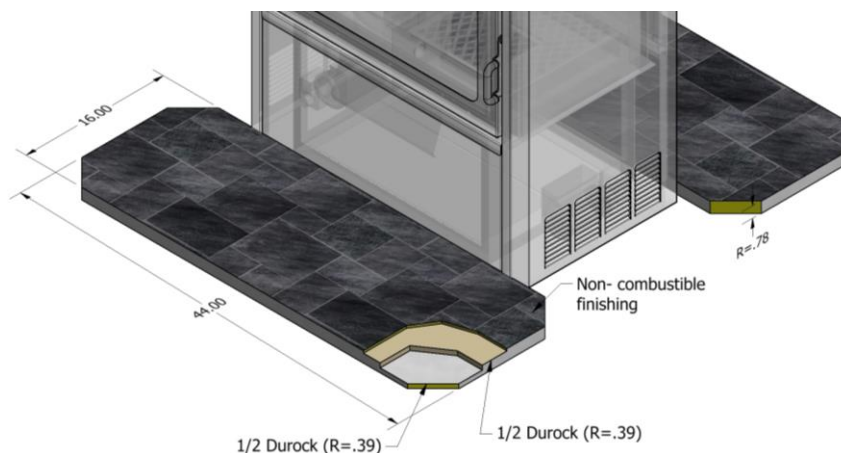
Figure 9.1 – Hearth Extension U.S.A
