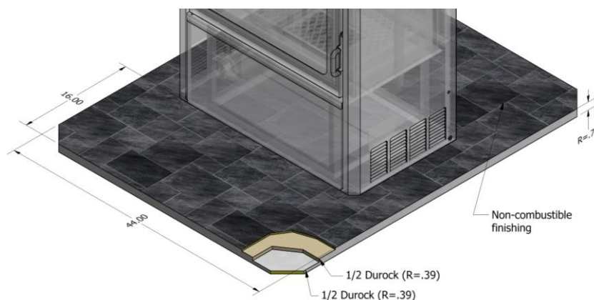
Figure 9.2 – Hearth Extension U.S.A
