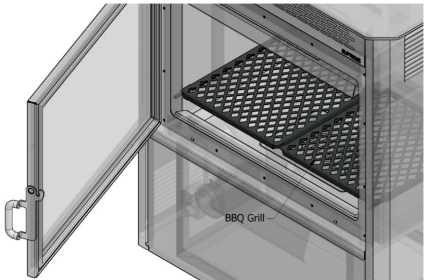
Figure 4 – Built-in Barbecue
