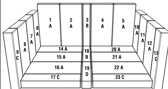
Firebox Brick Layout as Viewed from the Front
