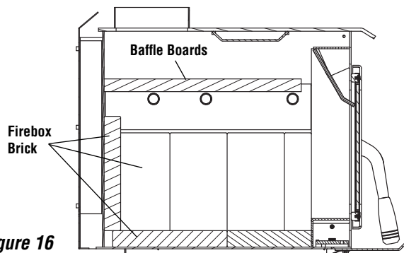
Side Cut-A-Way View of Firebox
