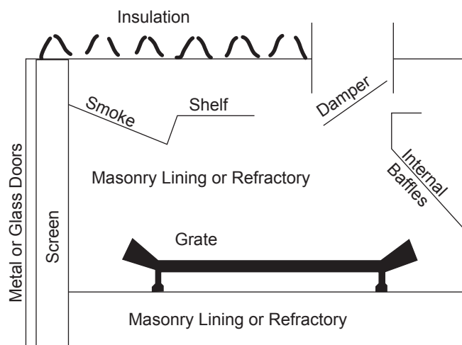
Figure 8 - Metal Fireplace Zero-Clearance Requirements
