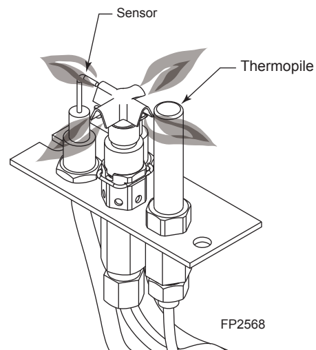
Figure 53 - Typical Pilot Flame
