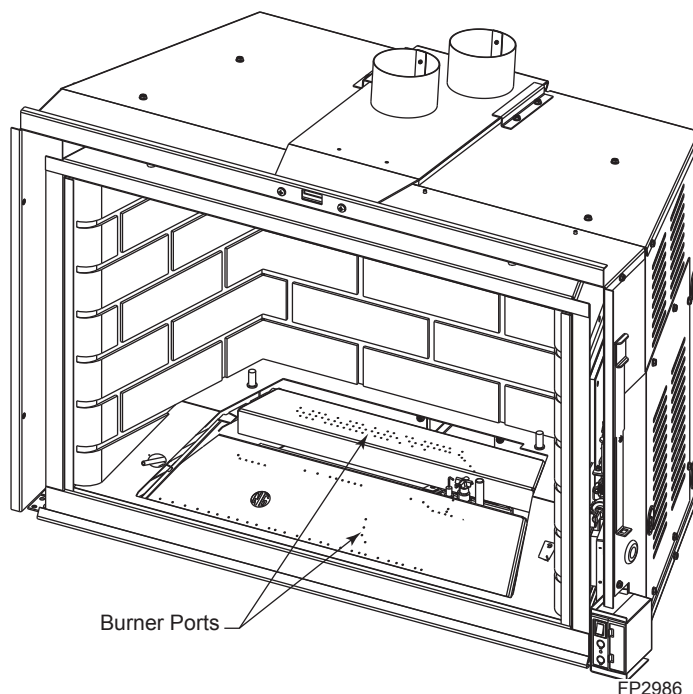
Figure 55 - Check Burner Ports and Burners
