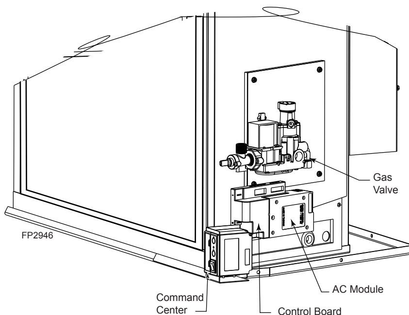
Figure 1 - 40ICFDV Series Fireplace Insert Controls
