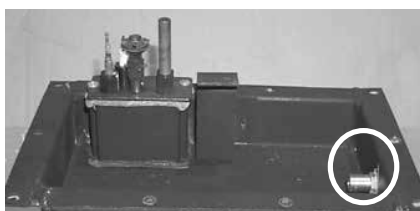
Burner Orifice
