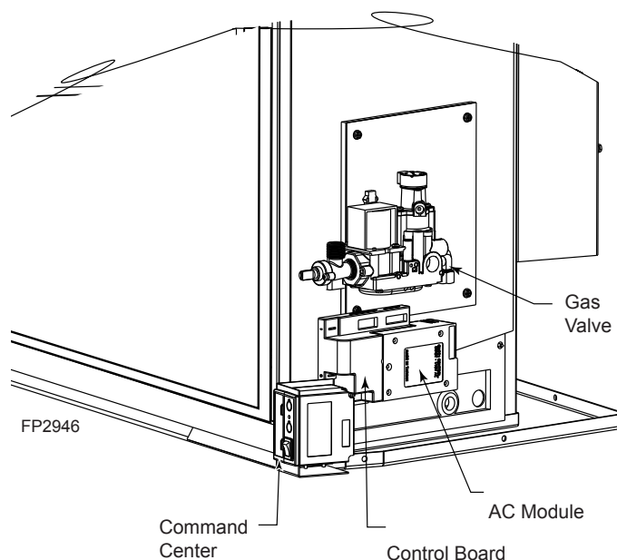
Figure 1 - VC41LDVI Series Fireplace Insert Controls
