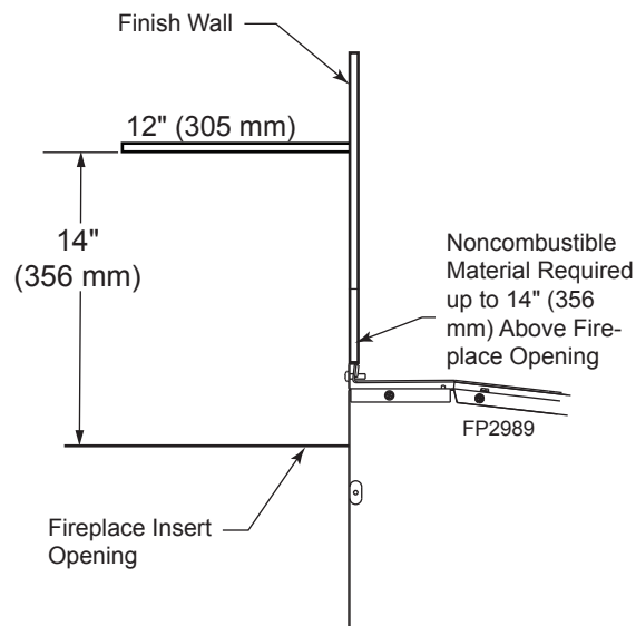
Figure 4 - Mantel Clearances
