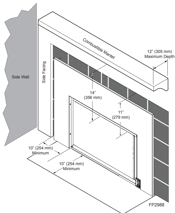
Figure 3 - Mantel Clearances
