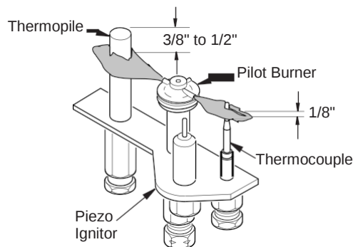
Figure 20 - Pilot Assembly
