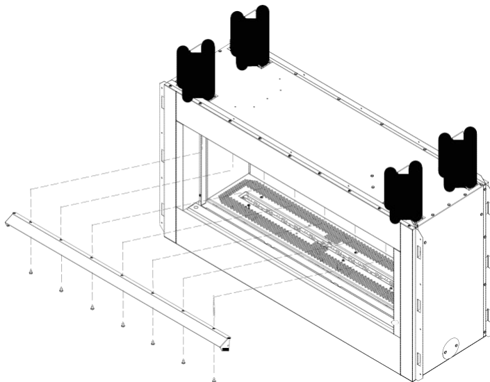
Figure 15 - Installing Hood
