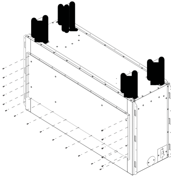
Figure 14 - Installing Rear Panel for Regular Applications
