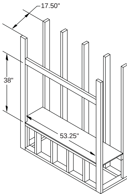
Figure 2 - Framing Clearances for One Sided Application
