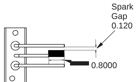
Figure 28 - Ignitor
