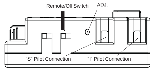
AF-4000 MOD Module Rt Side Figure 26 - Gas Module Right Side
