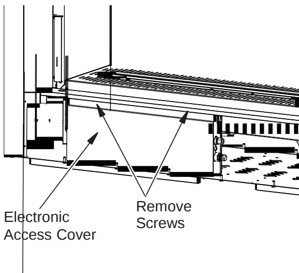
Figure 23 - Removing Control Access Cover (Face Bottom not shown for Clarity)
