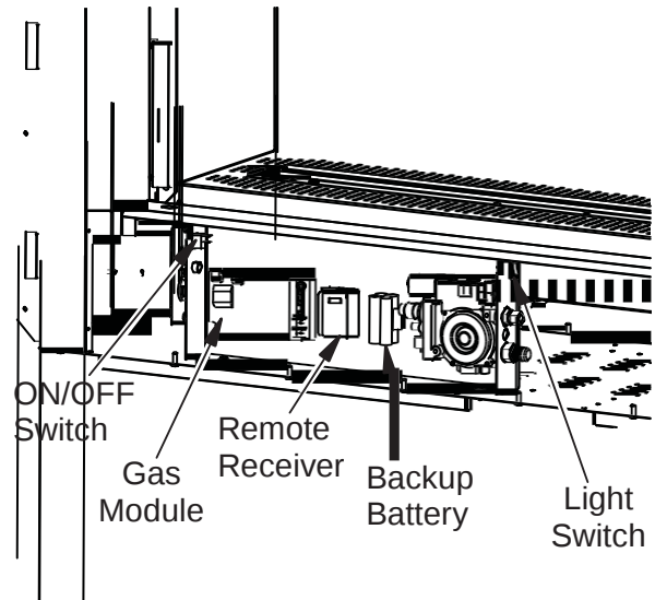
Figure 24 - Control Module (Face Bottom not shown for Clarity)
