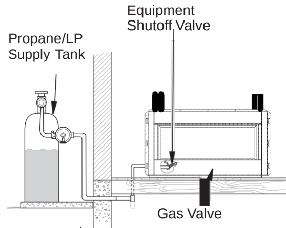
Figure 12 - Checking Gas Joints for Propane/LP Gas Fireplace
