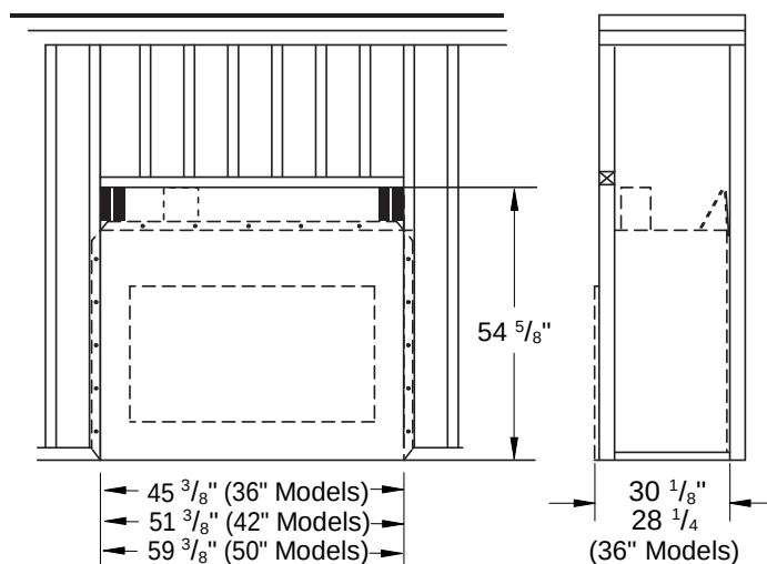
Figure 8 - Framing Dimensions
