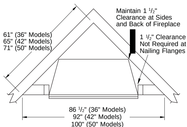
Figure 9 - Corner Installation
