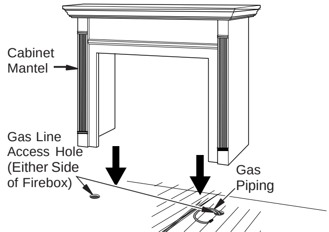
Figure 11 - Installing Cabinet Mantel (Mantel May Vary From Illustration)
