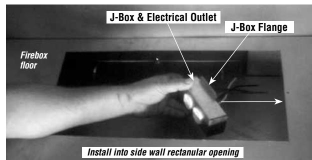
Figure 20 - Model VRT3542WS Shown
