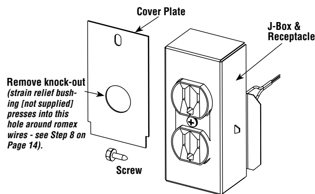
Figure 19 - Junction Box Kit (all models)
