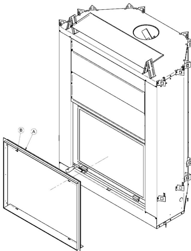
Figure 28.2 Masonry Trim
